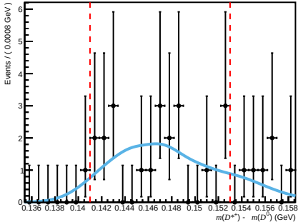
Passed ( 200 < nTracks < 600 , 3.6 < \eta < 5.0 , 10000 < p < 15600 )
