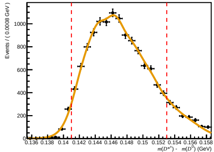
Total ( 200 < n\text{Tracks} < 600 , 3.6 < \eta < 5.0 , 10000 < p < 15600 )
