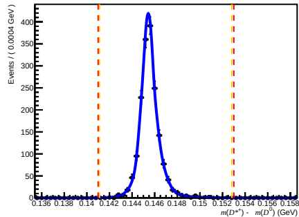
Failed DiF ( 0 < nTracks < 200 , 1.7 < \eta < 3.6 , 10000 < p < 15600 )
