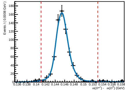
Total ( 0 < n\text{Tracks} < 200 , 3.6 < \eta < 5.0 , 10000 < p < 15600 )
