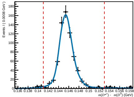
Passed ( 0 < n\text{Tracks} < 200 , 3.6 < \eta < 5.0 , 10000 < p < 15600 )
