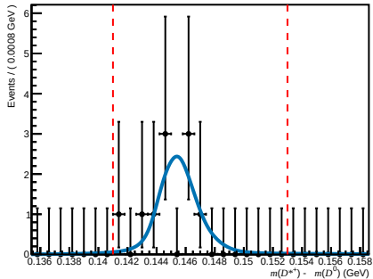
Failed ( 0 < n\text{Tracks} < 200 , 3.6 < \eta < 5.0 , 10000 < p < 15600 )
