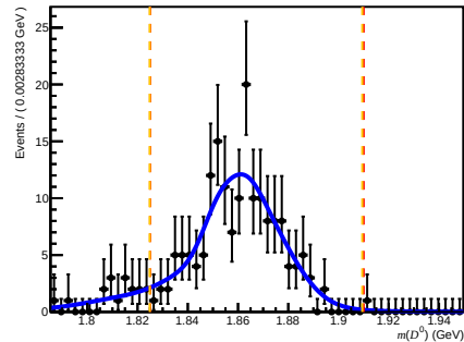
Failed Df ( 0 < n_{\text{Tracks}} < 200 , 3.6 < \eta < 5.0 , 60000 < p < 100000 )
