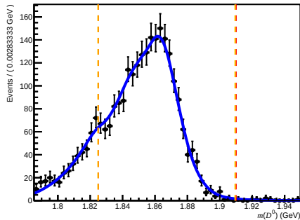
Passed Df (after RICH1) ( 0 < n_{\text{Tracks}} < 200 , 3.6 < \eta < 5.0 , 60000 < p < 100000 )
