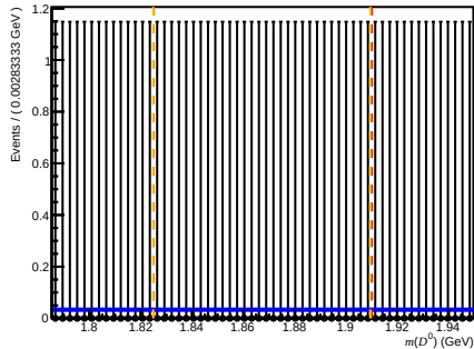
Passed Df (before RICH1) ( 0 < n_{\text{Tracks}} < 200 , 3.6 < \eta < 5.0 , 60000 < p < 100000 )
