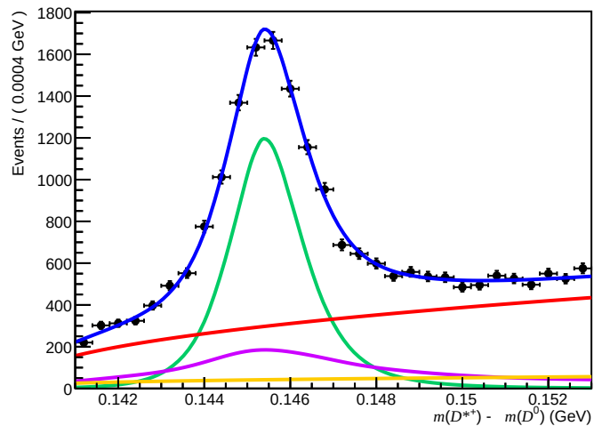
Passed ( 0 < n_{\text{Tracks}} < 200 , 3.6 < \eta < 5.0 , 60000 < p < 100000 )
