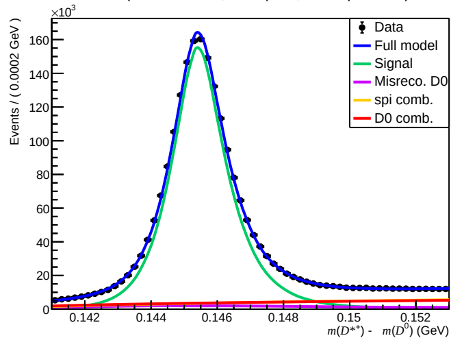
Failed ( 0 < n_{\text{Tracks}} < 200 , 3.6 < \eta < 5.0 , 60000 < p < 100000 )
