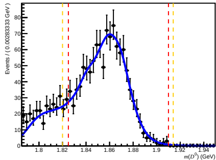
Passed DiF (after RICH1) ( 200 < n_{\text{Tracks}} < 600 , 3.6 < \eta < 5.0 , 10000 < p < 15600 )
