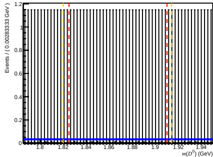
Passed DiF (before RICH1) ( 200 < n_{\text{Tracks}} < 600 , 3.6 < \eta < 5.0 , 10000 < p < 15600 )
