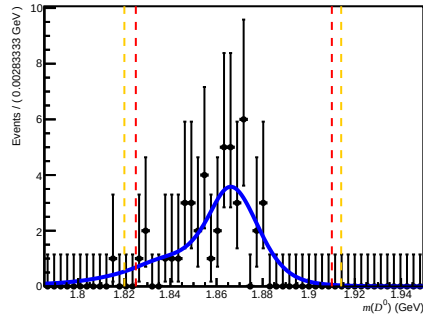
Failed DiF ( 200 < n_{\text{Tracks}} < 600 , 3.6 < \eta < 5.0 , 10000 < p < 15600 )
