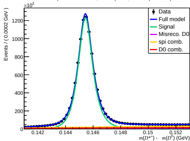
Failed ( 0 < n_{\text{Tracks}} < 200 , 1.7 < \eta < 3.6 , 10000 < p < 15600 )
