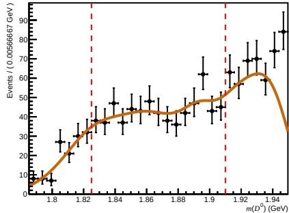
Failed ( 0 < nTracks < 200 , 3.6 < \eta < 5.0 , 6000 < p < 10000 )
