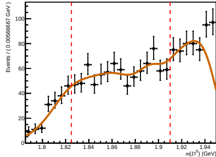
Total ( 0 < nTracks < 200 , 3.6 < \eta < 5.0 , 6000 < p < 10000 )
