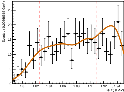
Passed ( 0 < nTracks < 200 , 3.6 < \eta < 5.0 , 6000 < p < 10000 )
