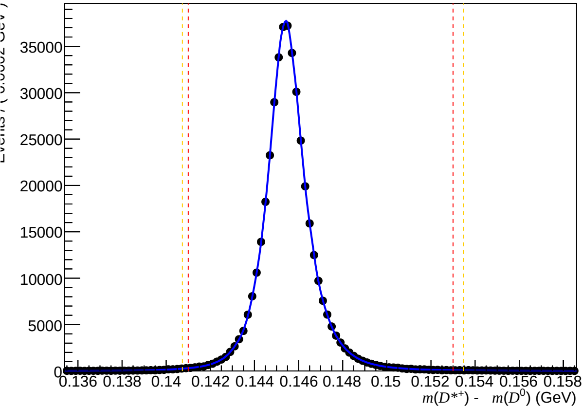
Failed non-DiF ( 0 < n\text{Tracks} < 200 , 3.6 < \eta < 5.0 , 6000 < p < 10000 )
