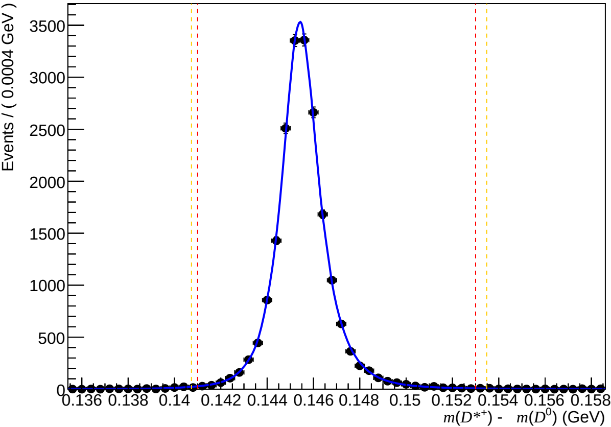
Passed non-DiF ( 0 < n\text{Tracks} < 200 , 3.6 < \eta < 5.0 , 6000 < p < 10000 )
