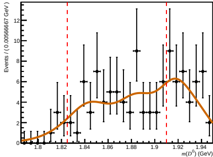
Passed ( 200 < nTracks < 600 , 1.7 < \eta < 3.6 , 3000 < p < 6000 )
