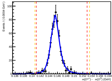
Passed DIF (after RICH1) ( 200 < nTracks < 600 , 3.6 < \eta < 5.0 , 6000 < p < 10000 )
