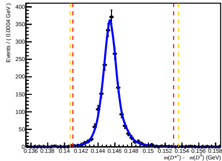
Failed DIF ( 200 < nTracks < 600 , 3.6 < \eta < 5.0 , 6000 < p < 10000 )
