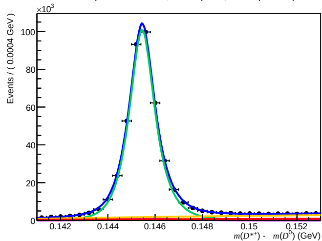
Passed ( 0 < n_{\text{Tracks}} < 200 , 1.7 < \eta < 3.6 , 3000 < p < 6000 )
