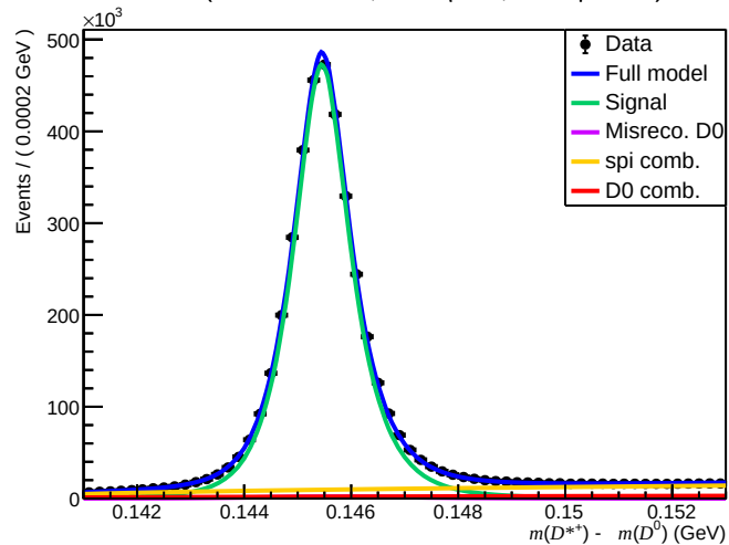
Failed ( 0 < n_{\text{Tracks}} < 200 , 1.7 < \eta < 3.6 , 3000 < p < 6000 )
