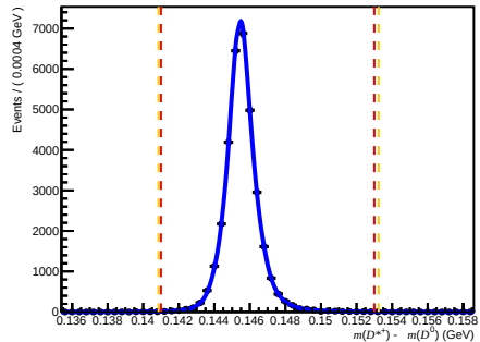
Passed DiF (after RICH1) ( 0 < nTracks < 200 , 1.7 < \eta < 3.6 , 15600 < p < 27000 )
