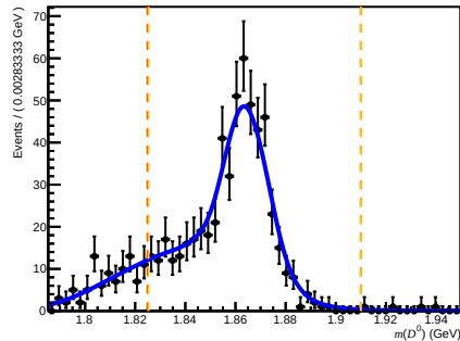
Failed DiF ( 0 < nTracks < 200 , 1.7 < \eta < 3.6 , 27000 < p < 60000 )
