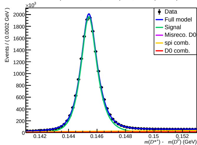
Failed ( 0 < nTracks < 200 , 1.7 < \eta < 3.6 , 27000 < p < 60000 )
