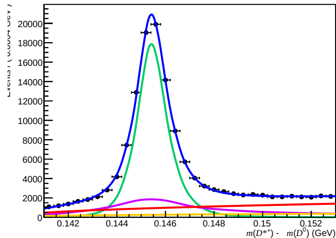
Failed ( 0 < nTracks < 200 , 1.7 < \eta < 3.6 , 27000 < p < 60000 )
