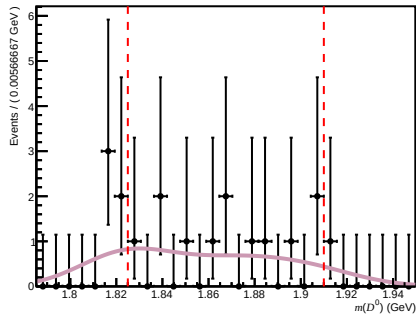
Total ( 0 < n\text{Tracks} < 200 , 3.6 < \eta < 5.0 , 10000 < p < 15600 )
