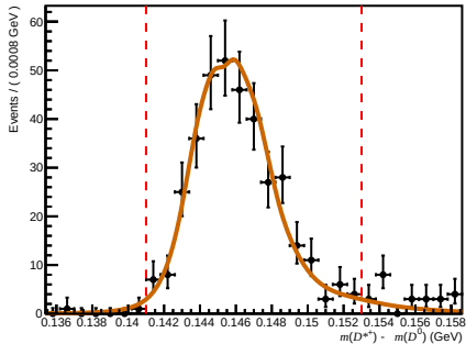
Passed ( 0 < nTracks < 200 , 3.6 < \eta < 5.0 , 27000 < p < 60000 )
