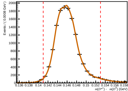
Total ( 0 < nTracks < 200 , 3.6 < \eta < 5.0 , 27000 < p < 60000 )
