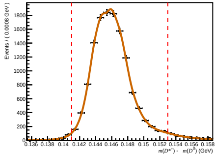
Failed ( 0 < nTracks < 200 , 3.6 < \eta < 5.0 , 27000 < p < 60000 )
