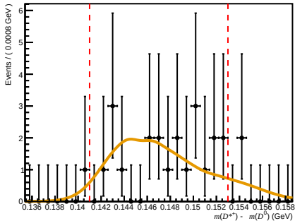
Passed ( 0 < nTracks < 200 , 3.6 < \eta < 5.0 , 60000 < p < 100000 )
