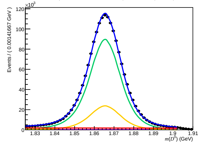
Failed ( 200 < n\text{Tracks} < 600 , 1.7 < \eta < 3.6 , 3000 < p < 6000 )
