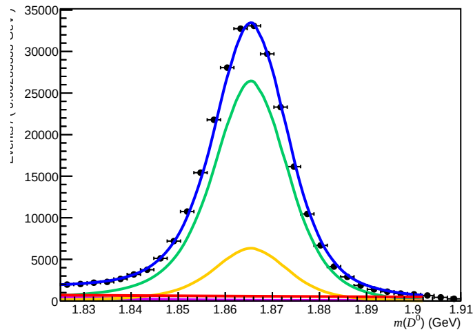
Passed ( 200 < n\text{Tracks} < 600 , 1.7 < \eta < 3.6 , 3000 < p < 6000 )
