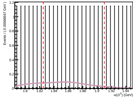
Passed ( 200 < nTracks < 600 , 1.7 < \eta < 3.6 , 6000 < p < 10000 )
