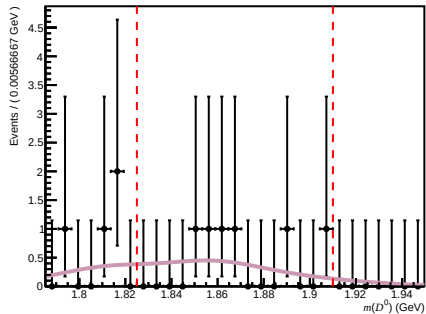
Failed ( 200 < nTracks < 600 , 1.7 < \eta < 3.6 , 6000 < p < 10000 )
