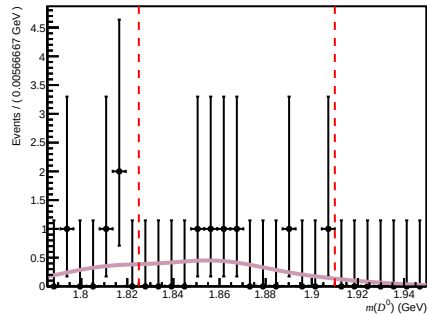
Total ( 200 < nTracks < 600 , 1.7 < \eta < 3.6 , 6000 < p < 10000 )
