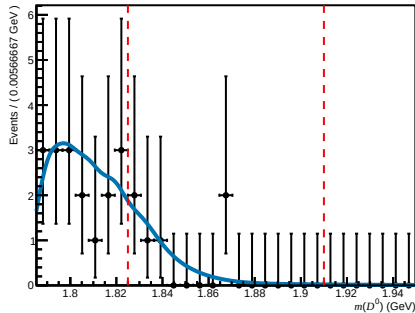
Failed ( 200 < n\text{Tracks} < 600 , 1.7 < \eta < 3.6 , 15600 < p < 27000 )
