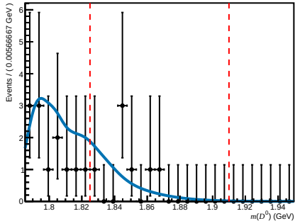
Failed ( 200 < nTracks < 600 , 3.6 < \eta < 5.0 , 3000 < p < 6000 )
