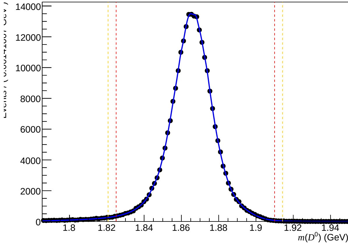
Failed non-DiF ( 200 < nTracks < 600 , 3.6 < \eta < 5.0 , 10000 < p < 15600 )
