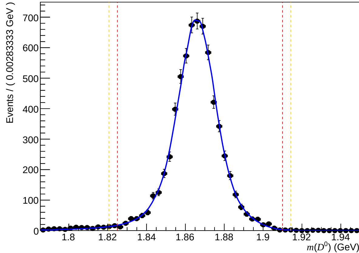
Passed non-DiF ( 200 < nTracks < 600 , 3.6 < \eta < 5.0 , 10000 < p < 15600 )
