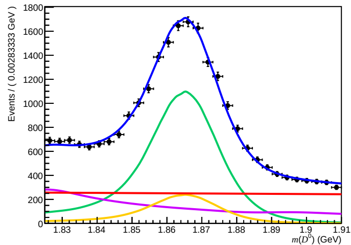
Passed (200 < nTracks < 600, 3.6 < \eta < 5.0, 60000 < p < 100000)
