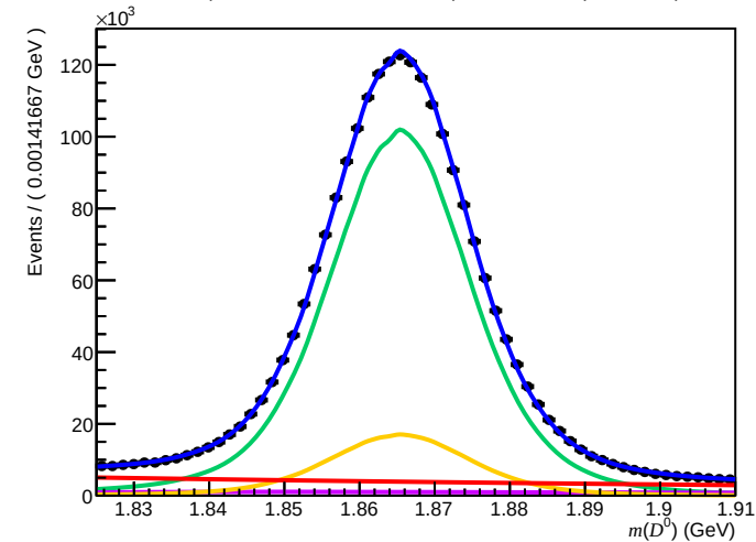
Failed (200 < nTracks < 600, 3.6 < \eta < 5.0, 60000 < p < 100000)
