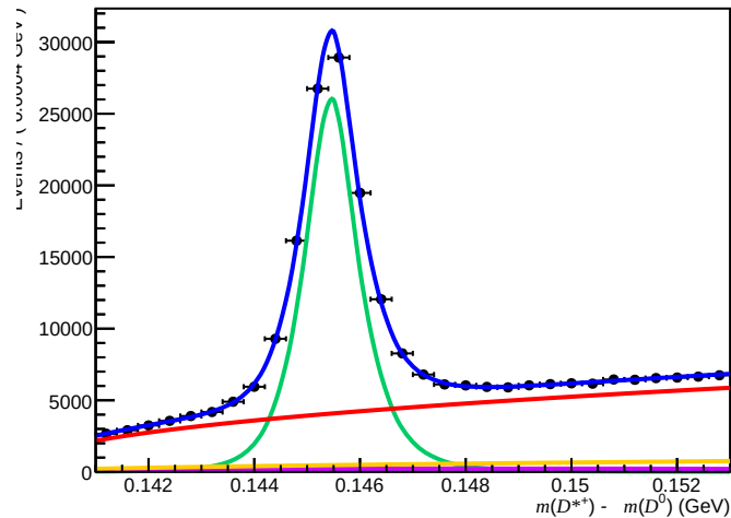
Failed ( 0 < n_{\text{Tracks}} < 200 , 1.7 < \eta < 3.6 , 3000 < p < 6000 )
