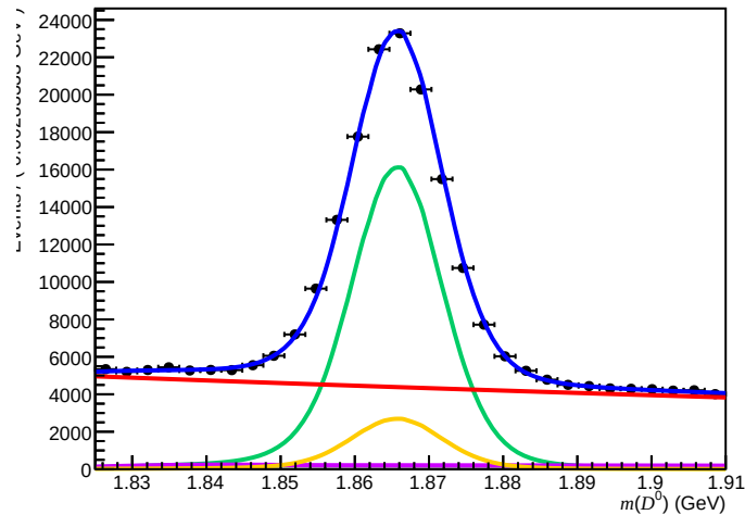
Failed ( 0 < n_{\text{Tracks}} < 200 , 1.7 < \eta < 3.6 , 3000 < p < 6000 )
