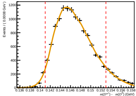
Failed ( 0 < n\text{Tracks} < 200 , 1.7 < \eta < 3.6 , 15600 < p < 27000 )
