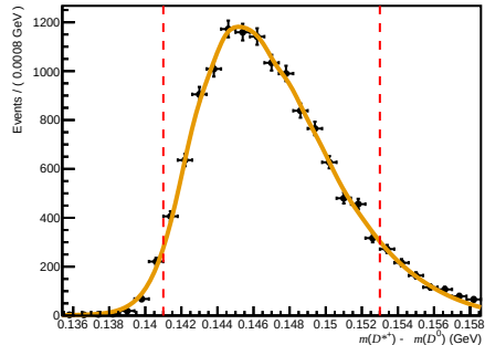
Total ( 0 < n\text{Tracks} < 200 , 1.7 < \eta < 3.6 , 15600 < p < 27000 )
