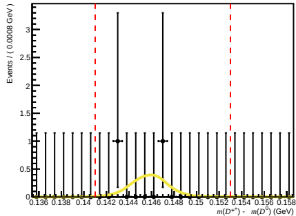
Passed ( 0 < nTracks < 200 , 1.7 < \eta < 3.6 , 27000 < p < 60000 )
