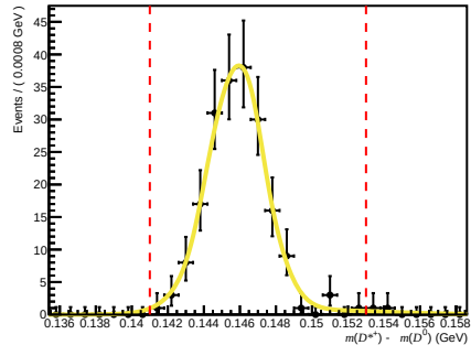
Total ( 0 < nTracks < 200 , 1.7 < \eta < 3.6 , 27000 < p < 60000 )
