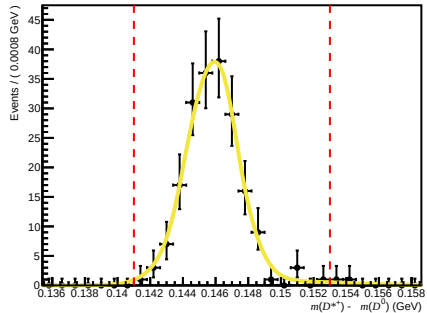
Failed ( 0 < nTracks < 200 , 1.7 < \eta < 3.6 , 27000 < p < 60000 )
