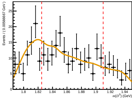
Passed ( 200 < nTracks < 600 , 1.7 < \eta < 3.6 , 10000 < p < 15600 )
