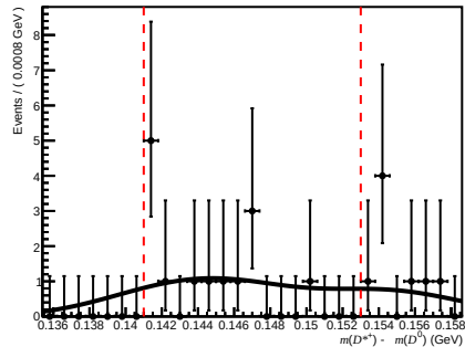
Total ( 200 < n\text{Tracks} < 600 , 1.7 < \eta < 3.6 , 27000 < p < 60000 )
