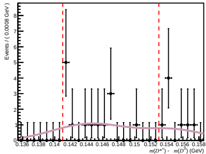
Failed ( 200 < n\text{Tracks} < 600 , 1.7 < \eta < 3.6 , 27000 < p < 60000 )
