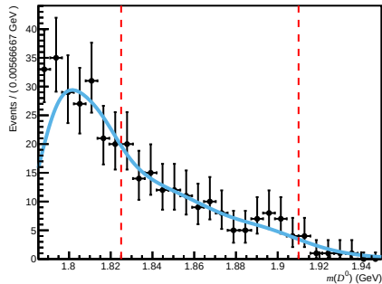
Total ( 200 < n\text{Tracks} < 600 , 1.7 < \eta < 3.6 , 60000 < p < 100000 )
