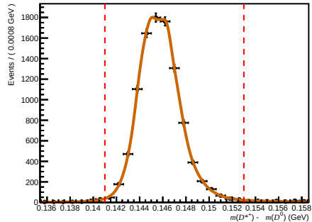
Failed ( 200 < nTracks < 600 , 1.7 < \eta < 3.6 , 60000 < p < 100000 )
