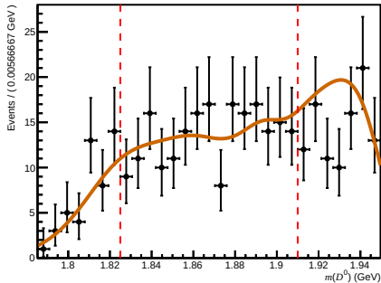
Passed ( 200 < n_{\text{Tracks}} < 600 , 3.6 < \eta < 5.0 , 6000 < p < 10000 )
