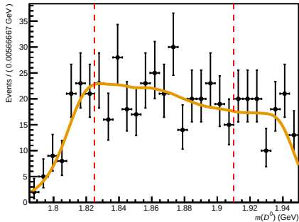
Passed ( 200 < nTracks < 600 , 3.6 < \eta < 5.0 , 6000 < p < 10000 )
