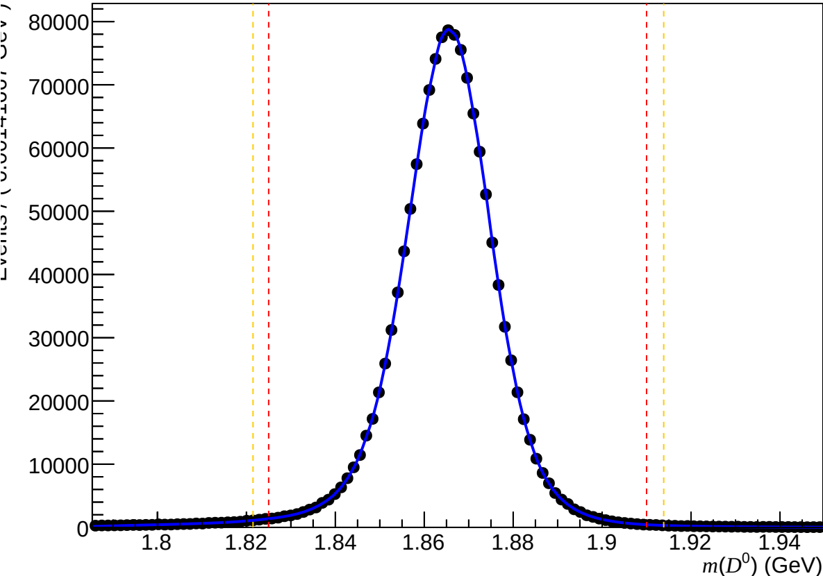
Failed non-DiF ( 200 < nTracks < 600 , 3.6 < \eta < 5.0 , 27000 < p < 60000 )
