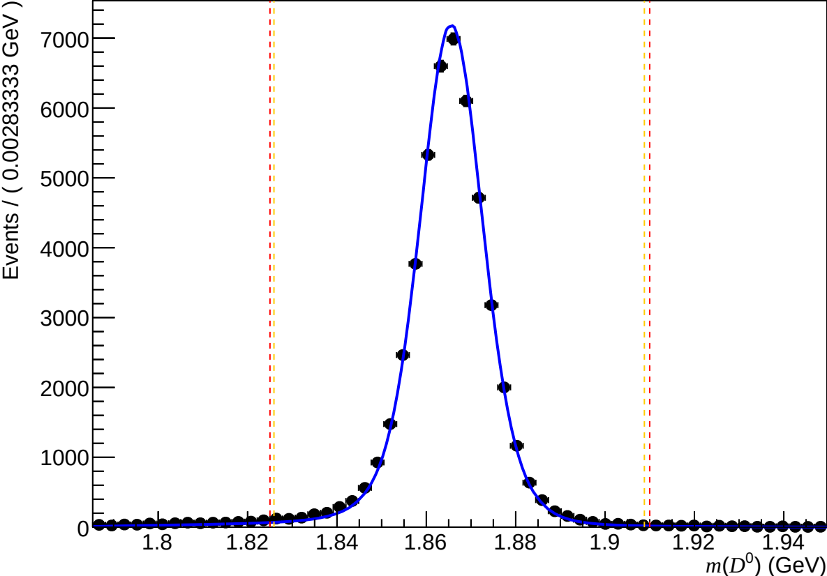
Passed non-DiF ( 0 < nTracks < 200 , 1.7 < \eta < 3.6 , 15600 < p < 27000 )
