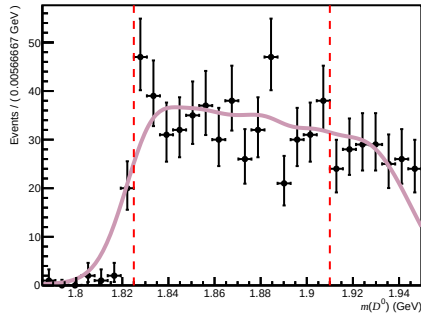
Total ( 0 < n_{\text{Tracks}} < 200 , 1.7 < \eta < 3.6 , 60000 < p < 100000 )
