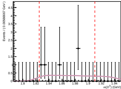
Passed ( 0 < n_{\text{Tracks}} < 200 , 1.7 < \eta < 3.6 , 60000 < p < 100000 )
