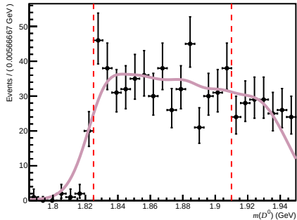
Failed ( 0 < n_{\text{Tracks}} < 200 , 1.7 < \eta < 3.6 , 60000 < p < 100000 )
