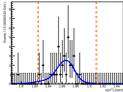
Failed DIF ( 0 < nTracks < 200 , 1.7 < \eta < 3.6 , 60000 < p < 100000 )
