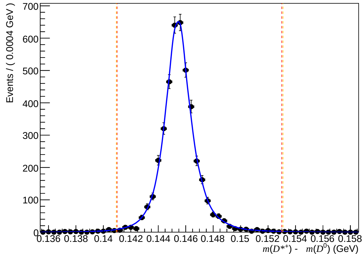
Passed non-DiF ( 0 < nTracks < 200 , 3.6 < \eta < 5.0 , 3000 < p < 6000 )
