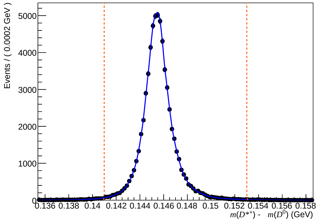
Failed non-DiF ( 0 < nTracks < 200 , 3.6 < \eta < 5.0 , 3000 < p < 6000 )
