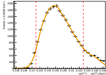
Total ( 0 < n\text{Tracks} < 200 , 3.6 < \eta < 5.0 , 27000 < p < 60000 )
