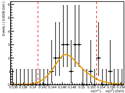
Passed ( 200 < n\text{Tracks} < 600 , 1.7 < \eta < 3.6 , 6000 < p < 10000 )
