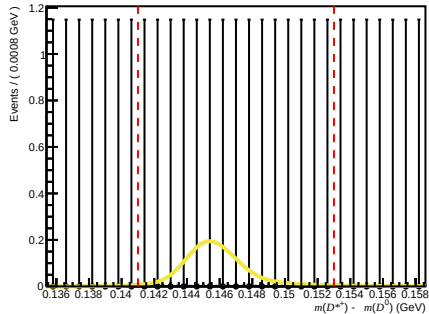
Passed ( 200 < n\text{Tracks} < 600 , 1.7 < \eta < 3.6 , 15600 < p < 27000 )
