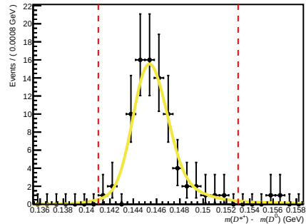
Total ( 200 < n\text{Tracks} < 600 , 1.7 < \eta < 3.6 , 15600 < p < 27000 )
