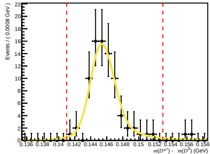
Failed ( 200 < n\text{Tracks} < 600 , 1.7 < \eta < 3.6 , 15600 < p < 27000 )
