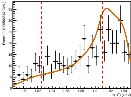
Passed ( 200 < nTracks < 600 , 1.7 < \eta < 3.6 , 27000 < p < 60000 )
