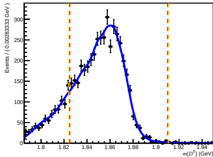
Passed DiF (after RICH1) ( 200 < n_{\text{Tracks}} < 600 , 1.7 < \eta < 3.6 , 27000 < p < 60000 )
