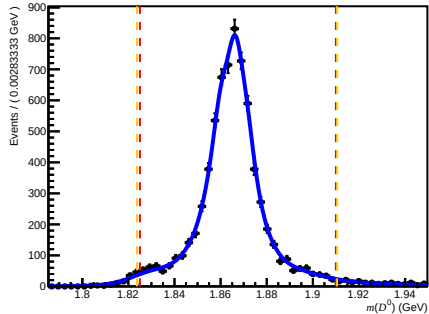
Passed DiF (after RICH1) ( 0 < n_{\text{Tracks}} < 200 , 1.7 < \eta < 3.6 , 3000 < p < 6000 )
