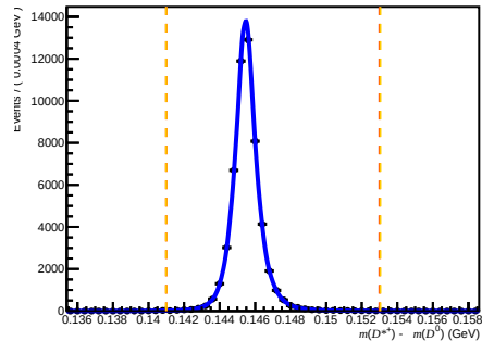
Failed DiF ( 0 < nTracks < 200 , 1.7 < \eta < 3.6 , 3000 < p < 6000 )
