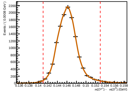
Total ( 0 < nTracks < 200 , 1.7 < \eta < 3.6 , 15600 < p < 27000 )
