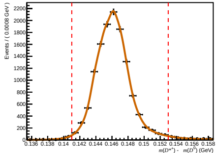
Failed ( 0 < nTracks < 200 , 1.7 < \eta < 3.6 , 15600 < p < 27000 )
