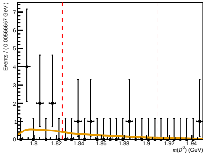
Passed ( 0 < nTracks < 200 , 3.6 < \eta < 5.0 , 27000 < p < 60000 )
