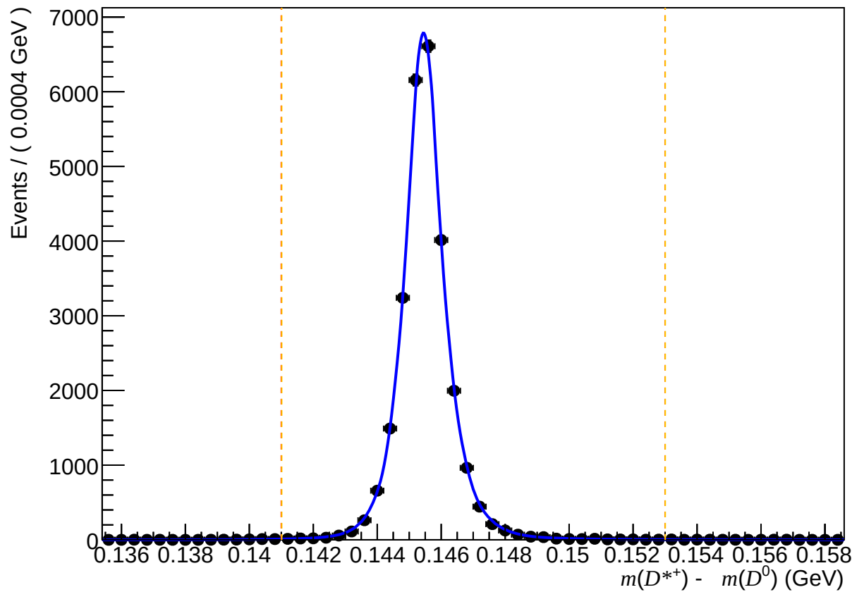
Passed non-DiF ( 200 < n\text{Tracks} < 600 , 1.7 < \eta < 3.6 , 3000 < p < 6000 )
