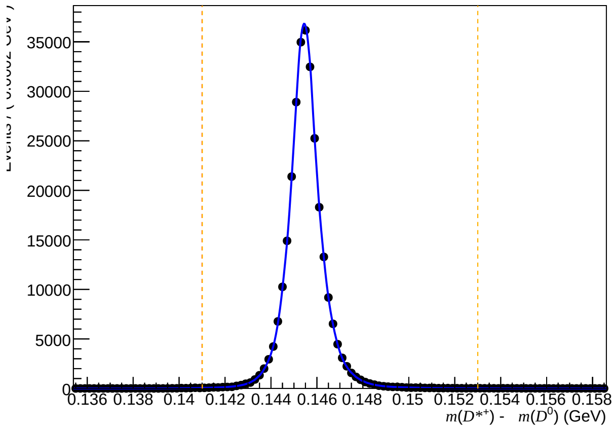
Failed non-DiF ( 200 < n\text{Tracks} < 600 , 1.7 < \eta < 3.6 , 3000 < p < 6000 )
